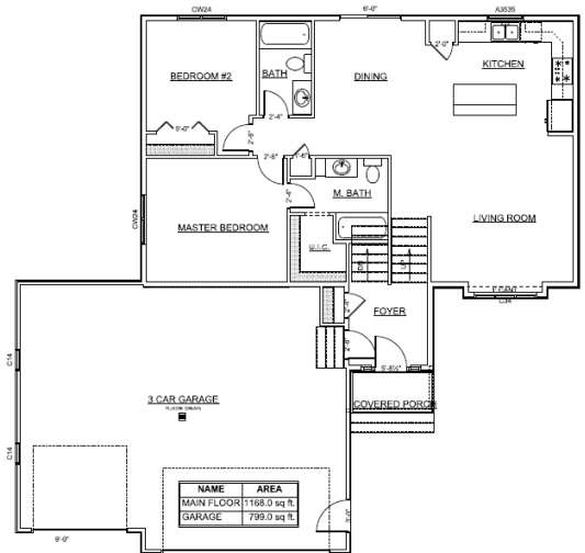
PHOENIX FLOOR PLAN SCALE = 1/8" = 1'-0"
