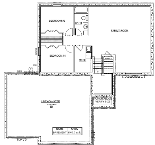
PHOENIX BASEMENT FLOOR PLAN SCALE = 1/8" = 1'-0"
