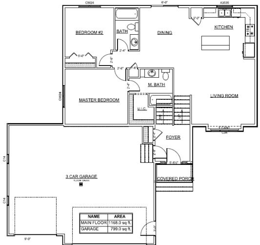
PHOENIX FLOOR PLAN SCALE = 1/8" = 1'-0"
