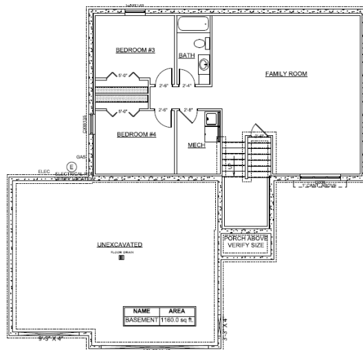
PHOENIX BASEMENT FLOOR PLAN
