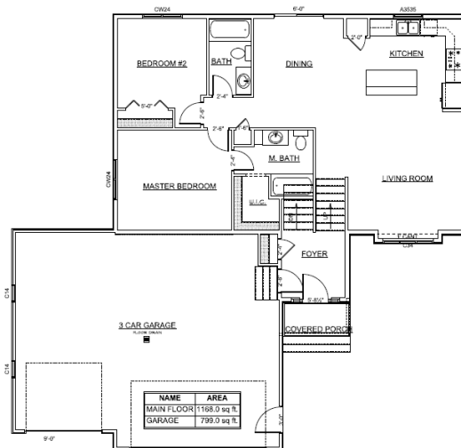
PHOENIX FLOOR PLAN
