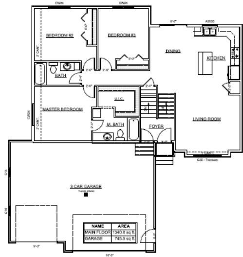
MONTEREY 01 FLOOR PLAN SCALE = 1/8" = 1'-0"
