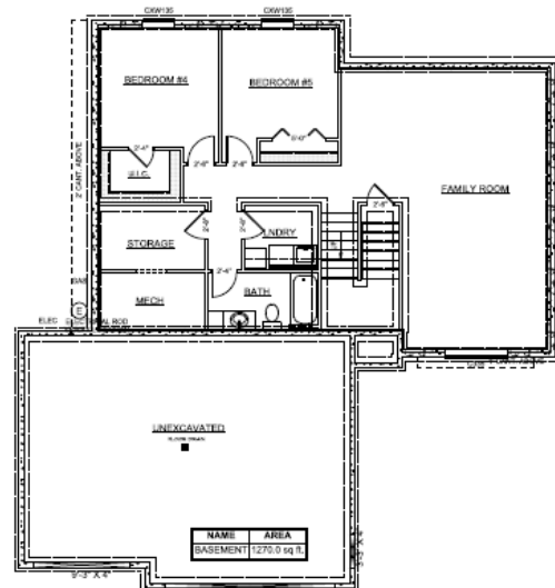
MONTEREY 01 BASEMENT FLOOR PLAN SCALE = 1/8" = 1'-0"
