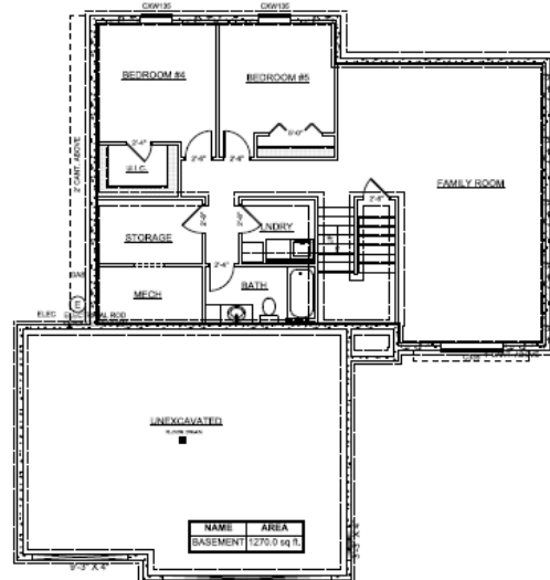
MONTEREY IN BASEMENT FLOOR PLAN SCALE = 1/8" = 1'-0"
