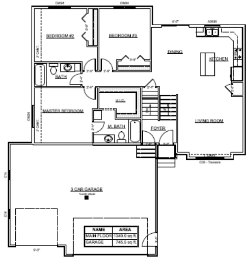
MONTEREY IN FLOOR PLAN SCALE = 1/8" = 1'-0"
