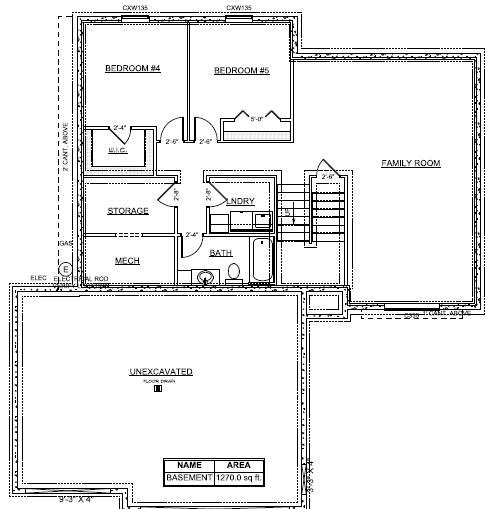
MONTEREY IN BASEMENT FLOOR PLAN SCALE = 1/8" = 1'-0"
