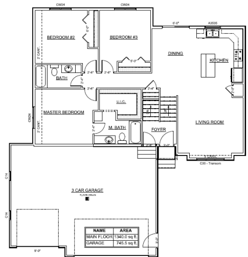
MONTEREY IN FLOOR PLAN SCALE = 1/8" = 1'-0"
